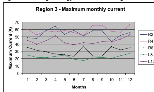
Figure 6 Maximum monthly current – Region 3.
