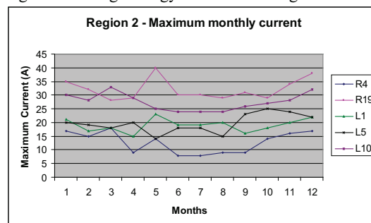
Figure 4 Maximum monthly current – Region 2.
