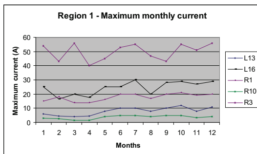
Figure 2 Maximum monthly current – Region 1.
